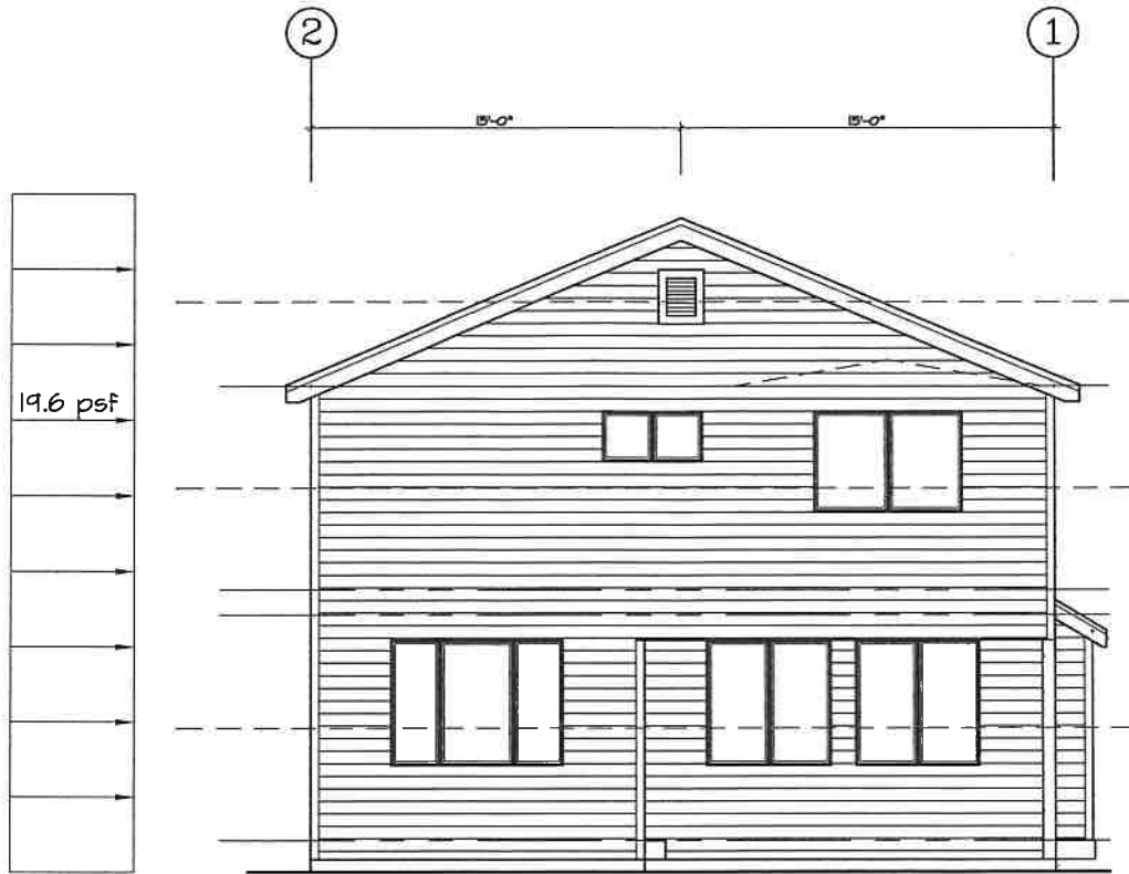
REAR ELEVATION
