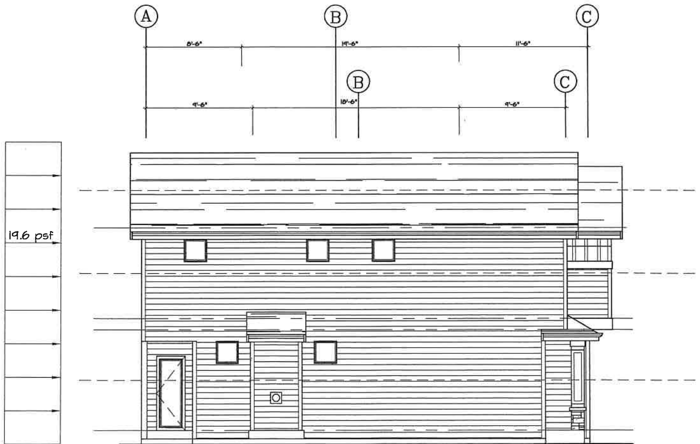
LEFT ELEVATION
